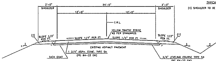
TYPICAL GRADING AND SURFACING SECTION NOTE: USE ASPHALT SAFETY EDGE. SEE SPECIAL PROVISION 411-14(a)-(b)09.
