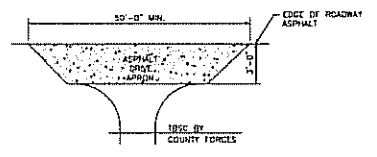
PLAN VIEW WIDENING FOR DRIVES (SEE STD. DET.-2 FOR DETAILS OF DRIVES)
